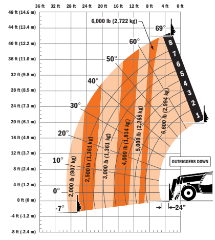
642 With Outriggers
