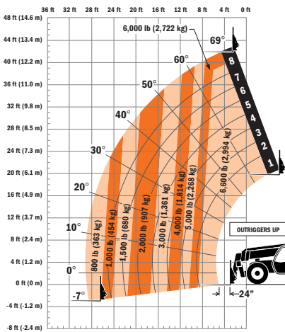
642 With Outriggers
